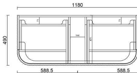
Top View 1200mm
