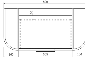
Top View 900mm
