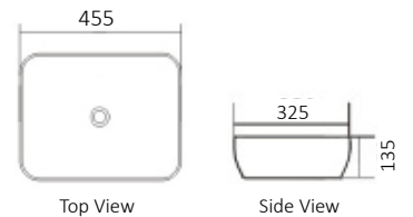
Top View Side View Ultra Slim Fine Ceramic Requires 32mm Waste, No Overflow Dimension 455 x 325 x 135mm Pop Up Wastes Sold Separately
