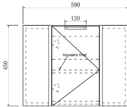
Front View Door Only
