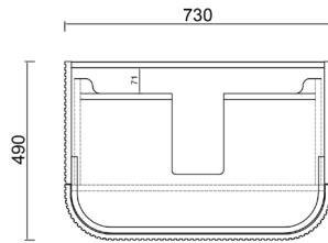
Top View 750mm
